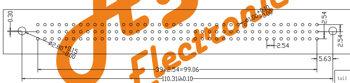
Recommended P.C.B.Layout
